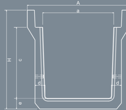
SECTION
